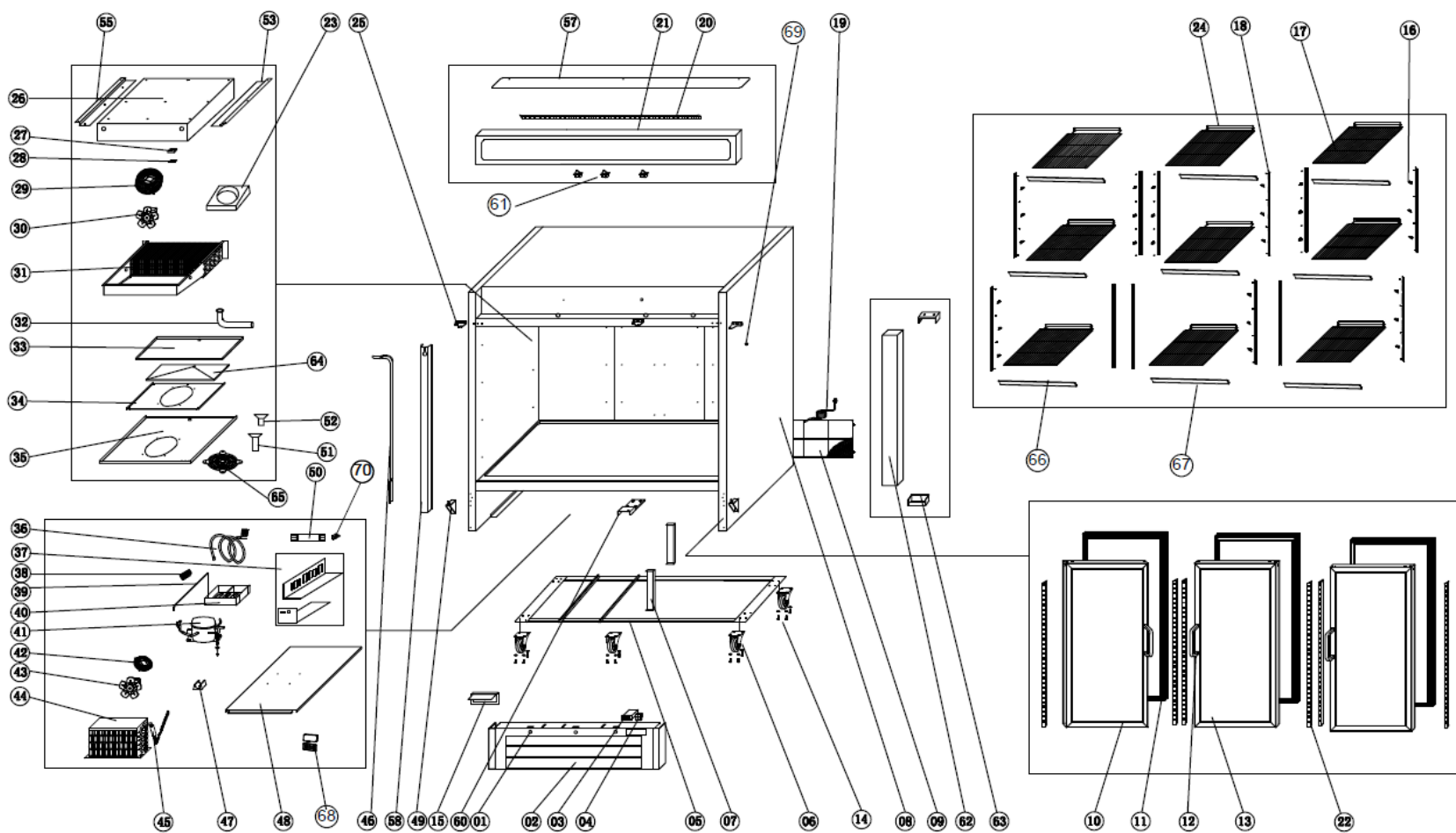
EXPLODE OF KCHGM72R
